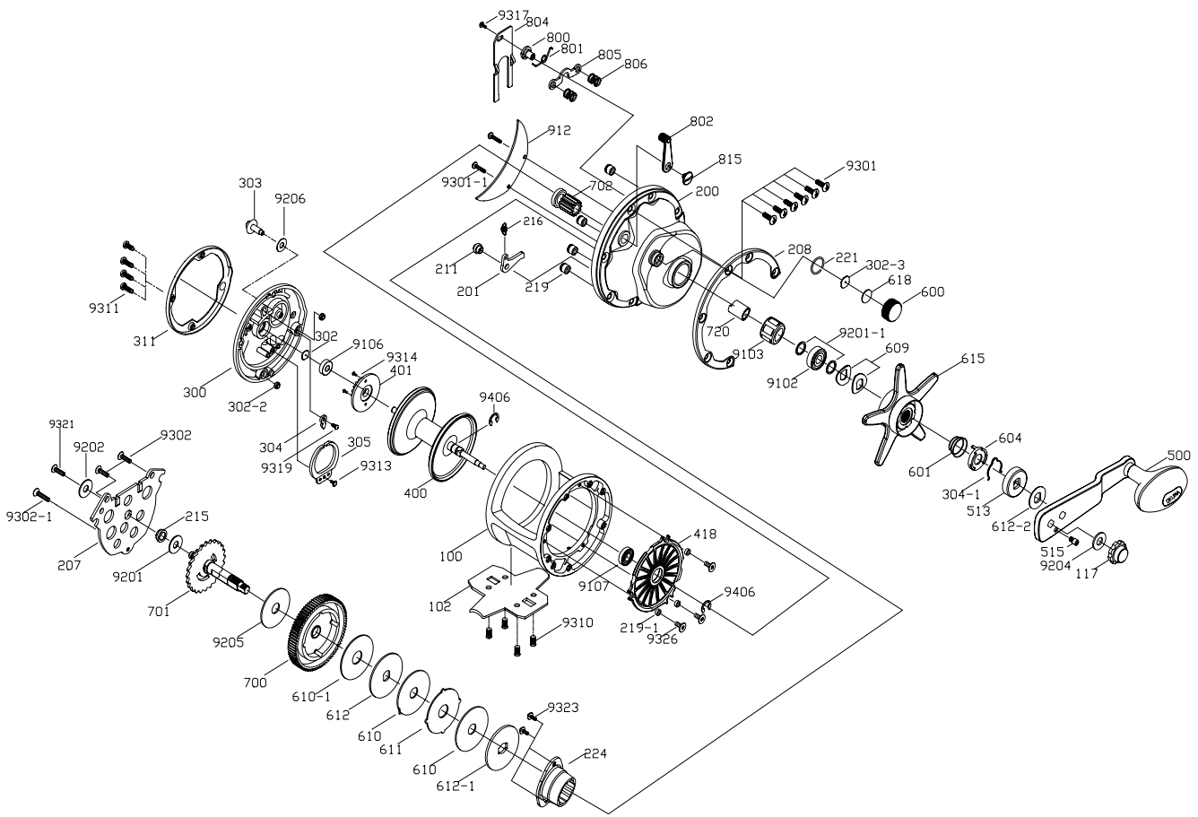
CT - 25CS Spare Parts
